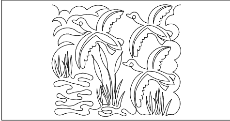
Duck Marsh
