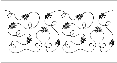
Ant's Picnic
