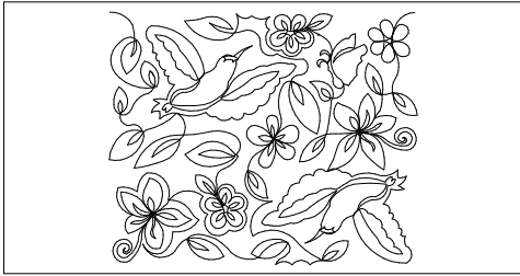
Hummingbirds
